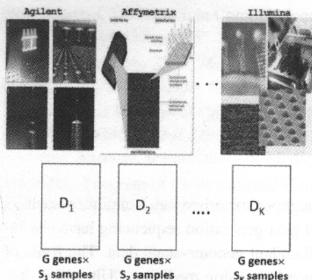
Figure I.1 (A) Horizontal omics meta-analysis. (B) Vertical multi-omics integrative analysis.
