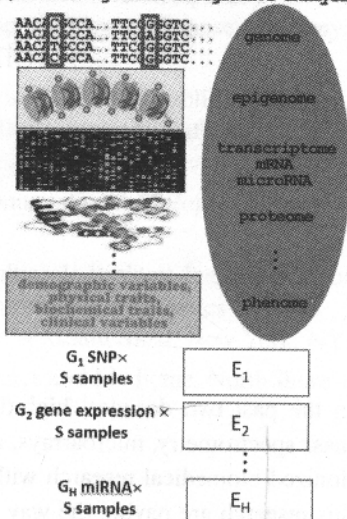
Figure I.1 (A) Horizontal omics meta-analysis. (B) Vertical multi-omics integrative analysis.
